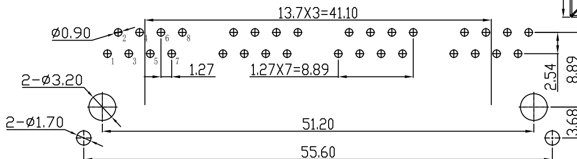
PC Board Layout
