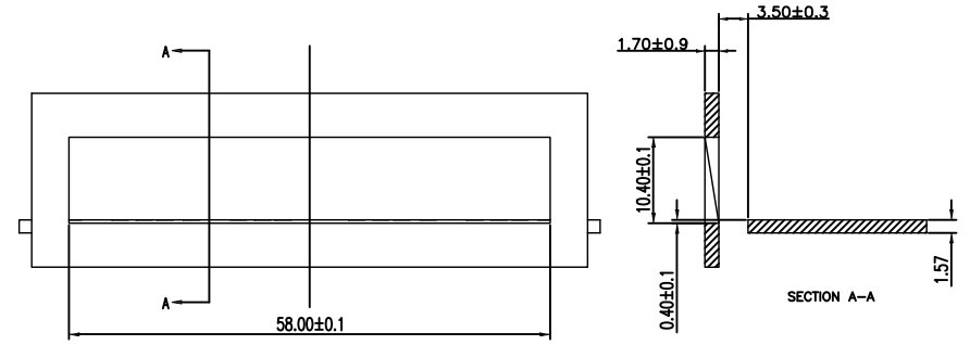
RECOMMENDED BEZEL DESIGN
