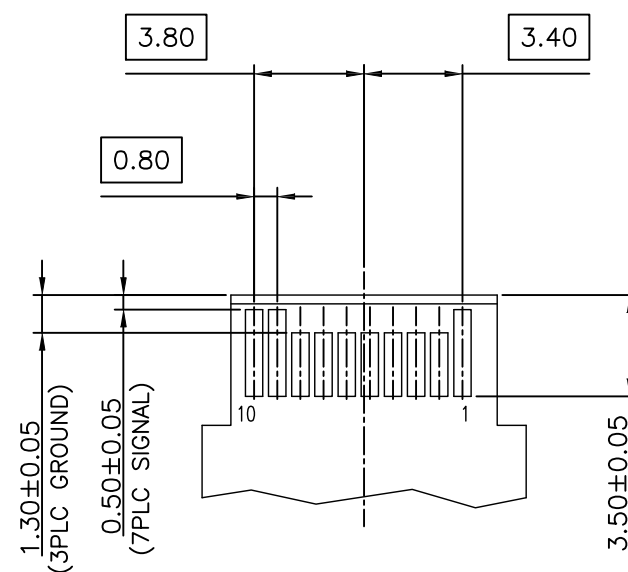
BOTTOM VIEW OF BOARD
