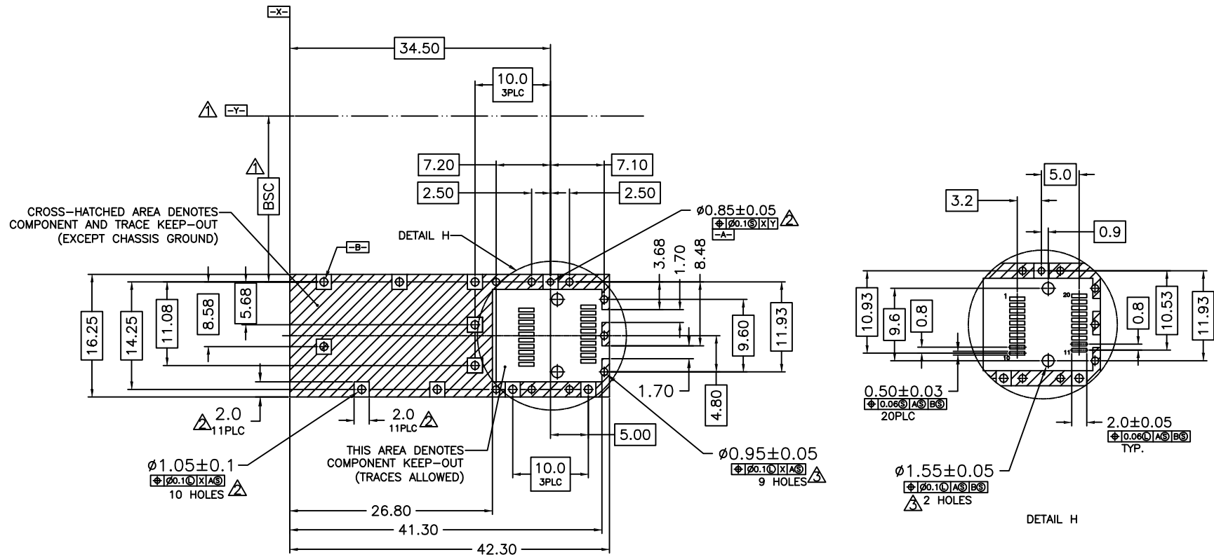
RECOMMENDED PCB CONFIGURATION
