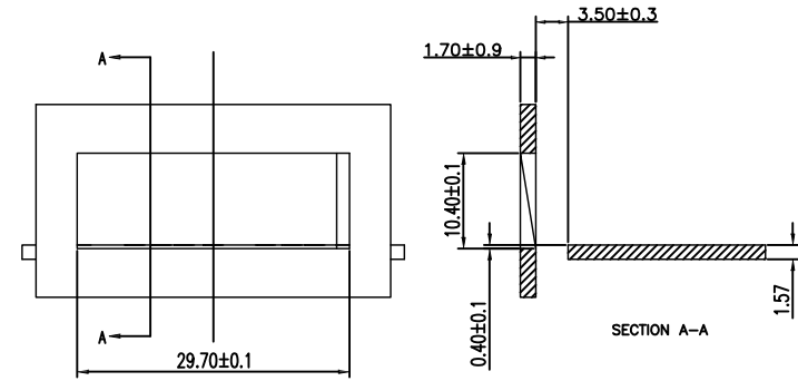
RECOMMENDED BEZEL DESIGN
