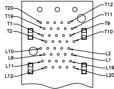
CONNECTOR PIN-OUT COMPONENT SIDE OF BOARD
