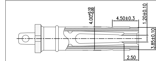
MATING PLUG P/N.:DP400170-0001-60000H
