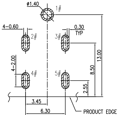
RECOMMENDED PCB LAYOUT(T=1.00) TOP VIEW TOLERANCE:±0.05
