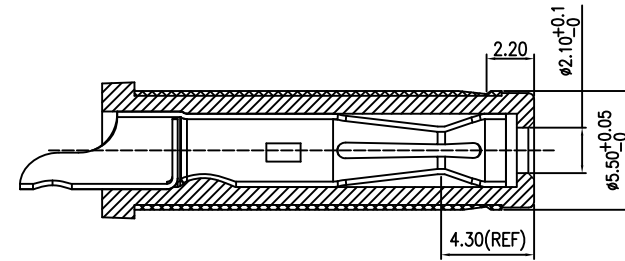
MATING PLUG DP550200-0129-60000H
