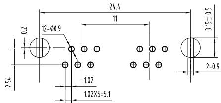
PC Board Layout Component Side Shown
