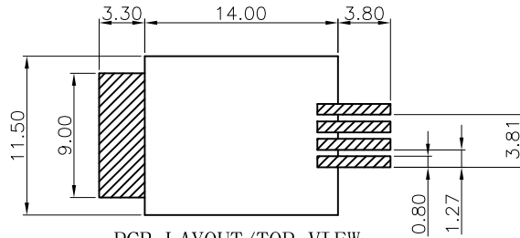
PCB LAYOUT/TOP VIEW TOLERANCE=± 0.05
