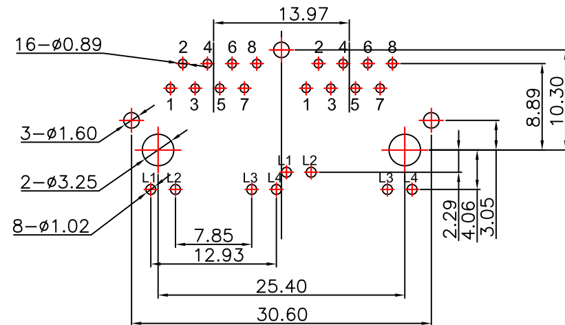
Recommended PCB Layout (Tolerance: \pm 0.05 )
