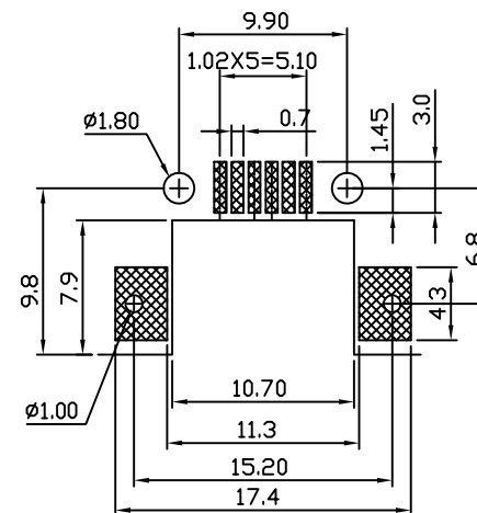
P.C.B. Layout (TOP VIEW)t=1
