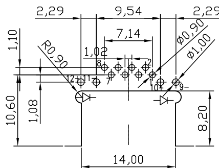
PCB LAYOUT TOP VIEW TOL: ±0.05
