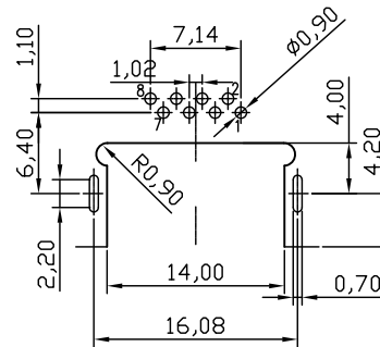
PCBLAYOUT TOP VIEW TOL:±0.05
