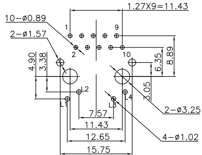
Suggested PCB Layout(Top View) (Tolerance:±0.05)
