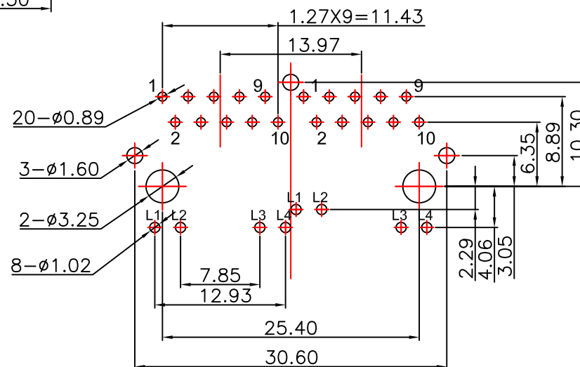
Recommended PCB Layout (Tolerance: \pm 0.05 )
