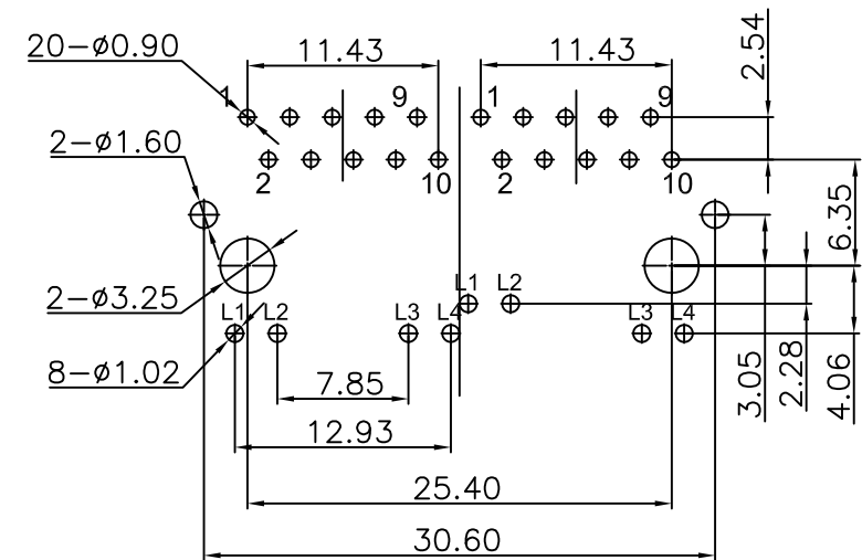
Recommended PCB Layout (Tolerance:±0.05)
