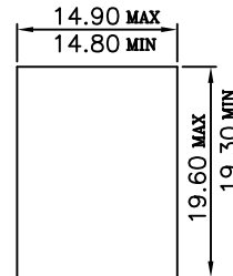
Single Panel-Latch Clearance Panel Thickness 1.20mm
