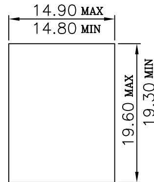
Single Panel-Latch Clearance Panel Thickness 1.60mm
